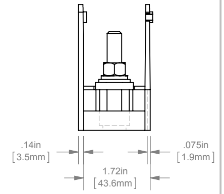
BACK VIEW ADDER (MPDB66200) SHOWN
