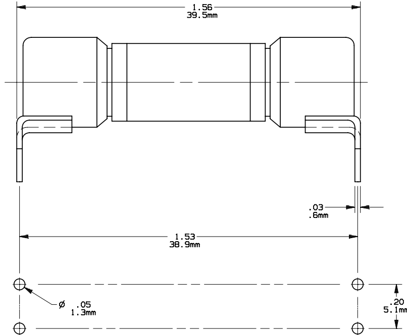
MOUNTING HOLE DETAIL
