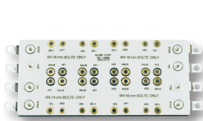
HIGH FREQUENCY WELDING BUS BAR
