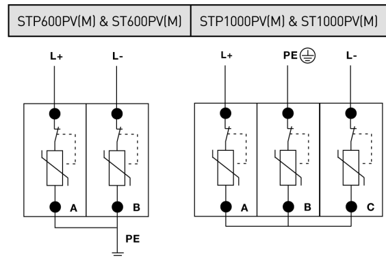
Figure 4: Wiring Diagram
