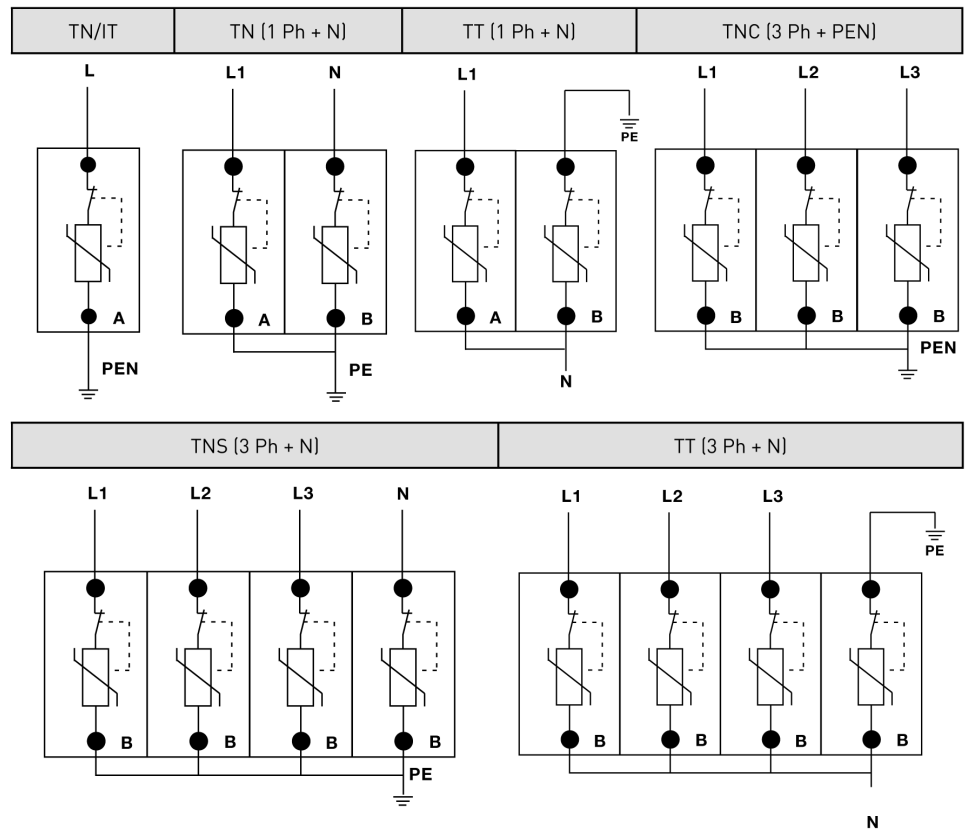
Figure 4: Wiring Diagram
