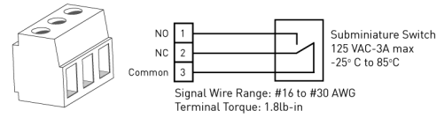
Figure 3: Microswitch
