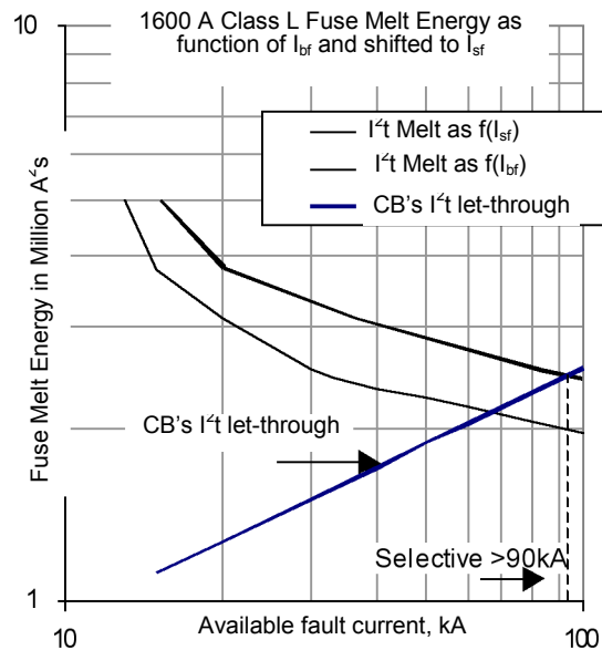
Fig. 13. A fuse's required melt energy as a function of I_{bf} and I_{sf} and the downstream circuit breaker's let-through energy.
