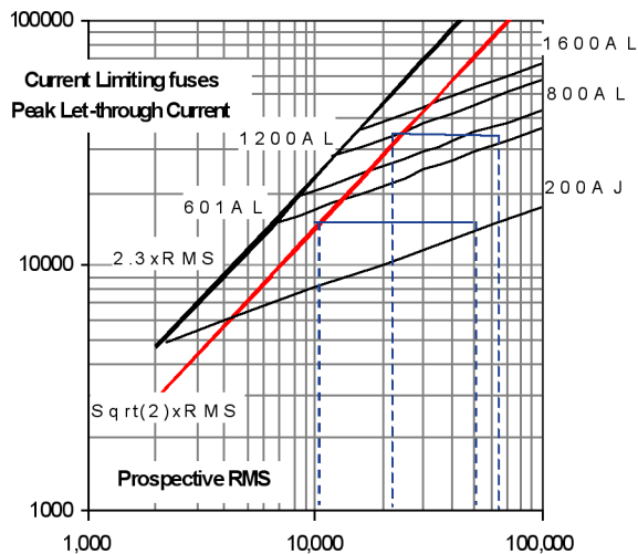
Fig. 5. Peak current let-through for several current-limiting fuses.
